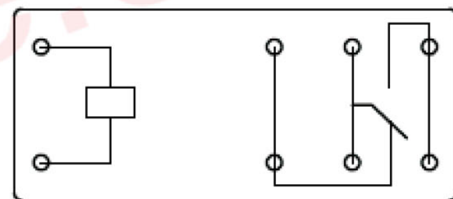
Conversion C type
