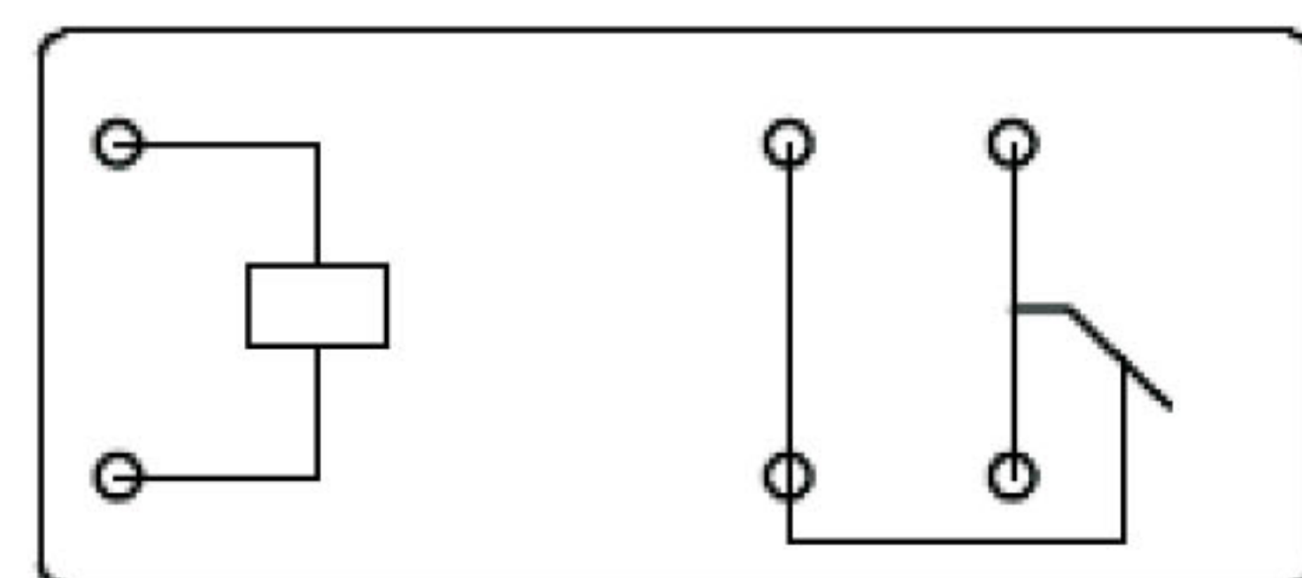
Normally closed B type
